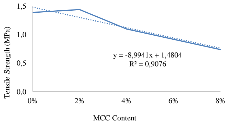
Figure 2. Tensile Strength Profile for 60% Glycerol Samples
